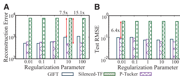
Fig. 6. Performance comparisons of GIFT, Silenced-TF and P-Tucker. (A) is a reconstruction error plot. (B) is a test RMSE plot
